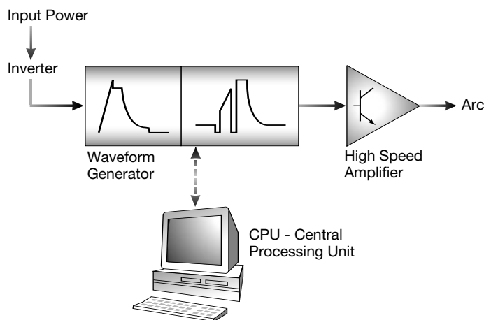
FIGURE 12: Wave Designer 2000 Pulse Editor
