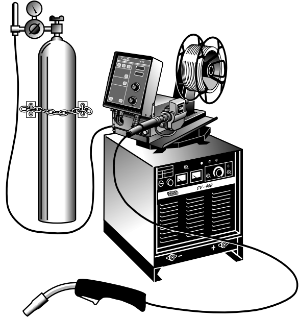
FIGURE 19: CV-400 with LN-10 GMAW System
