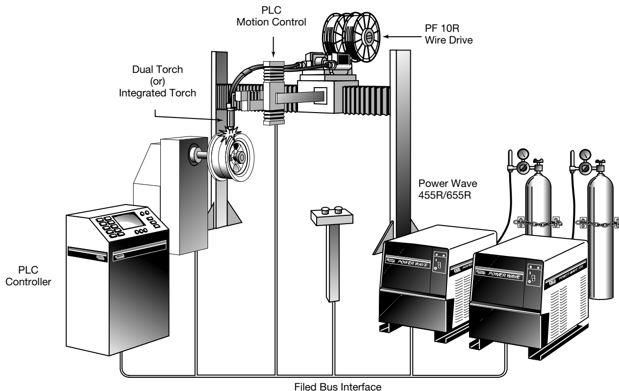
FIGURE 15: Tandem GMAW System
