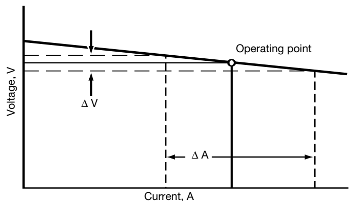
FIGURE 23: CV (Constant Voltage) Power Source Volt-Amp Characteristics
