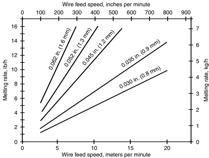
FIGURE 42: Typical Melting Rates for Carbon and Low Alloy Steel Electrodes
