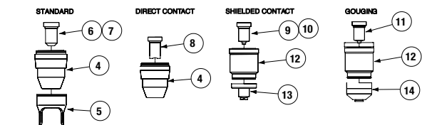
LC65 Optional Nozzles & Related Accessories
