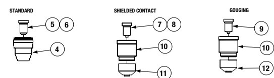
LC65M Optional Nozzles & Related Accessories
